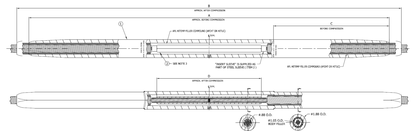
Figure 18: AFL Compression Splice Assembly.
